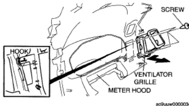
Fig. 21: Identifying Ventilator Grille With Hook & Screw - Driver Side Courtesy of MAZDA MOTORS CORP.
