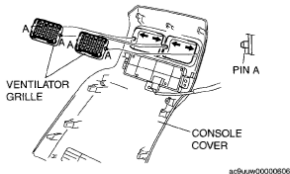
Fig. 24: Identifying Ventilator Grille & Center Panel With Screw - Rear Courtesy of MAZDA MOTORS CORP.
