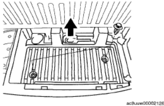
Fig. 70: Identifying Trunk Box With Clips Courtesy of MAZDA MOTORS CORP.
