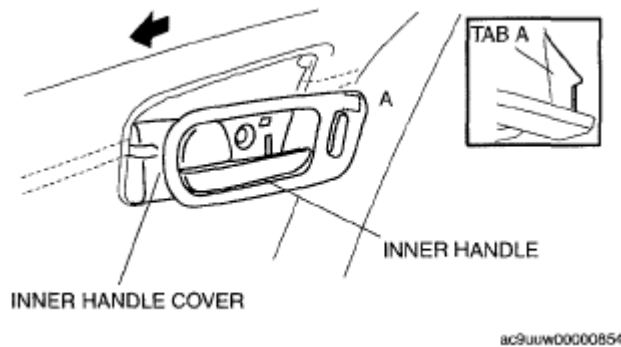
Fig. 64: Identifying Inner Handle & Cover Courtesy of MAZDA MOTORS CORP.
