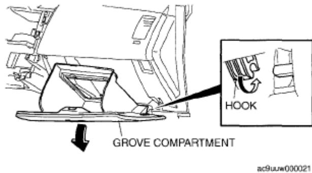
Fig. 20: Identifying Glove Compartment With Hook Courtesy of MAZDA MOTORS CORP.
