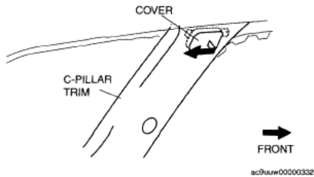
Fig. 50: Identifying C-Pillar Trim & Cover Courtesy of MAZDA MOTORS CORP.
