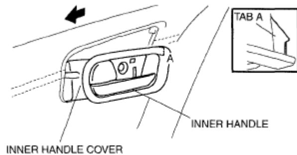
Fig. 68: Identifying Inner Handle & Cover Courtesy of MAZDA MOTORS CORP.
