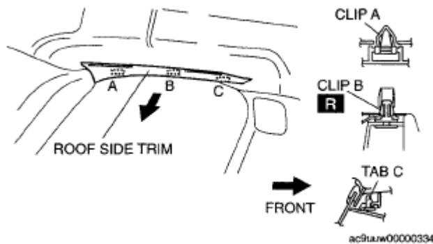
Fig. 49: Identifying Roof Side Trim & Clips Courtesy of MAZDA MOTORS CORP.
