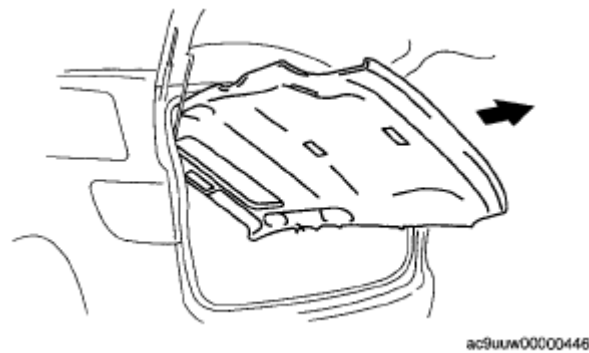
Fig. 83: Identifying Headliner Courtesy of MAZDA MOTORS CORP.
