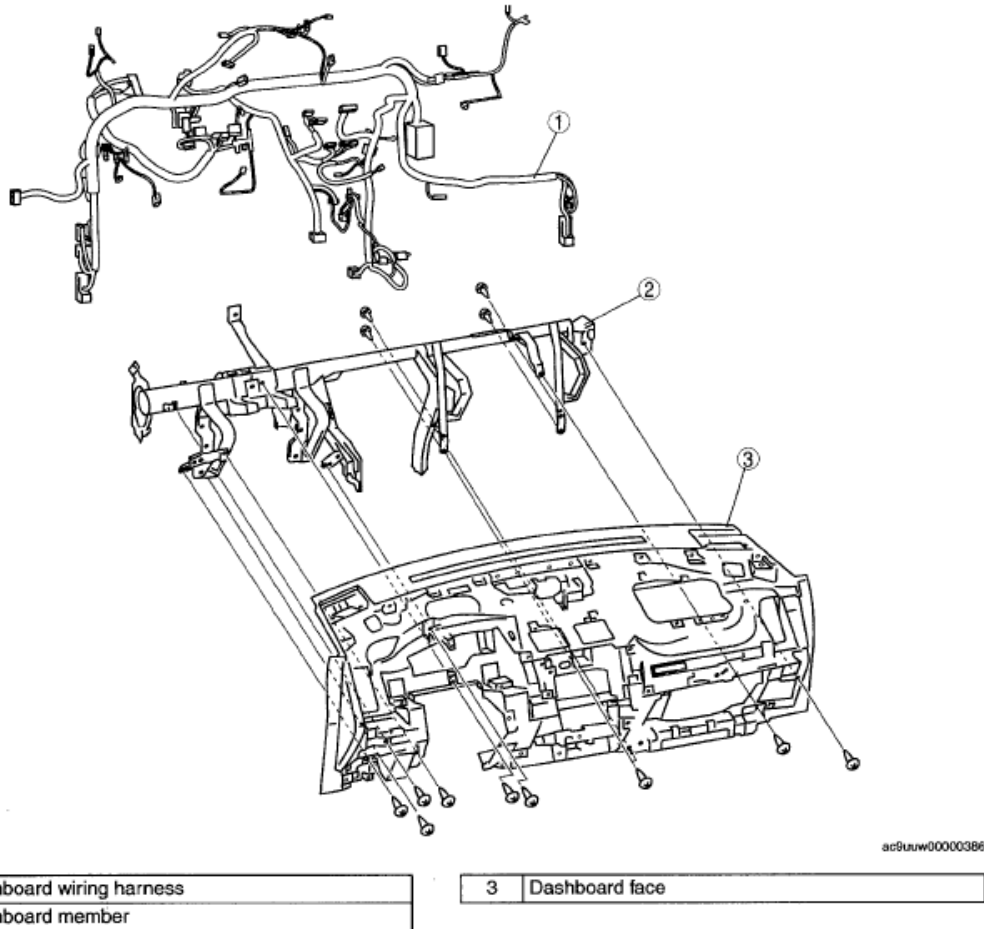
Fig. 6: Identifying Dashboard Wiring Harness, Member & Dashboard Face Courtesy of MAZDA MOTORS CORP.
