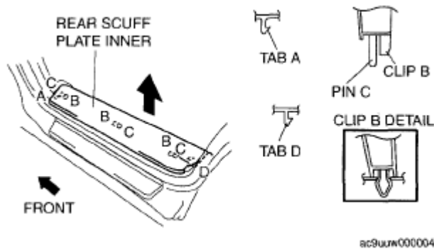
Fig. 56: Identifying Rear Scuff Plate Inner With Tab & Clips Courtesy of MAZDA MOTORS CORP.
