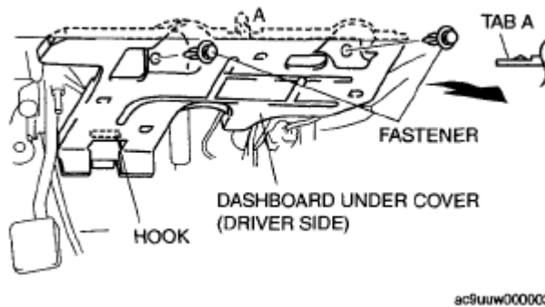
Fig. 27: Identifying Dashboard Under Cover, Hook & Clips (Driver Side) Courtesy of MAZDA MOTORS CORP.
