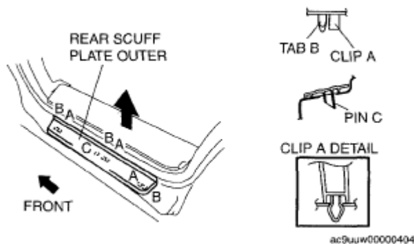
Fig. 57: Identifying Rear Scuff Plate Outer With Tab & Clips Courtesy of MAZDA MOTORS CORP.
