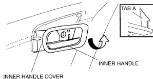
Fig. 69: Turning Inner Handle Cover Courtesy of MAZDA MOTORS CORP.
