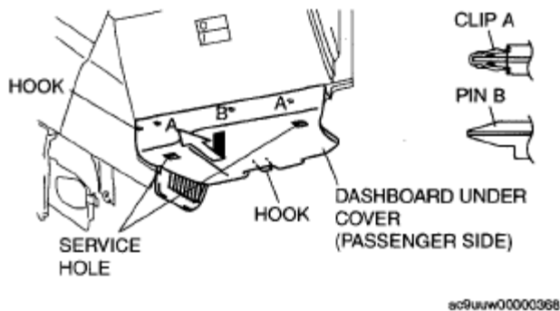
Fig. 28: Identifying Dashboard Under Cover, Hook & Clips (Passenger Side) Courtesy of MAZDA MOTORS CORP.
