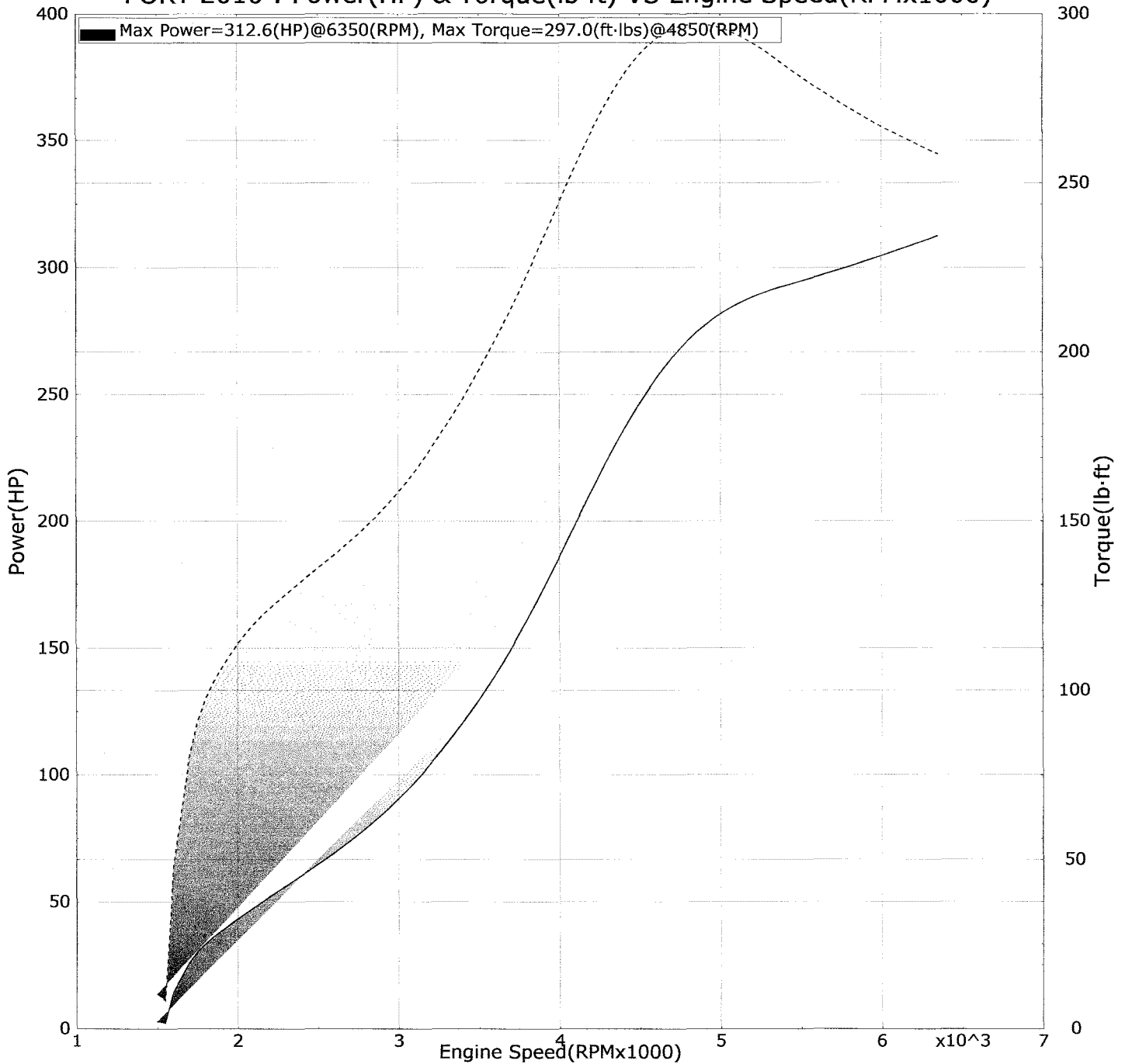
PORT 2010 : Power(HP) & Torque(lb-ft) VS Engine Speed(RPMx1000)
